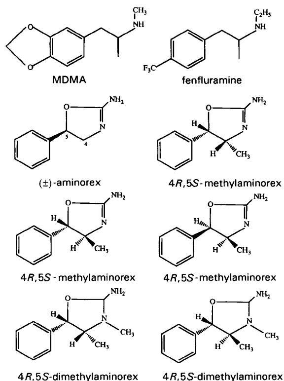
FIG. 1. The chemical structure of MDMA, fenfluramine and aminorex analogues used in the experiment.
